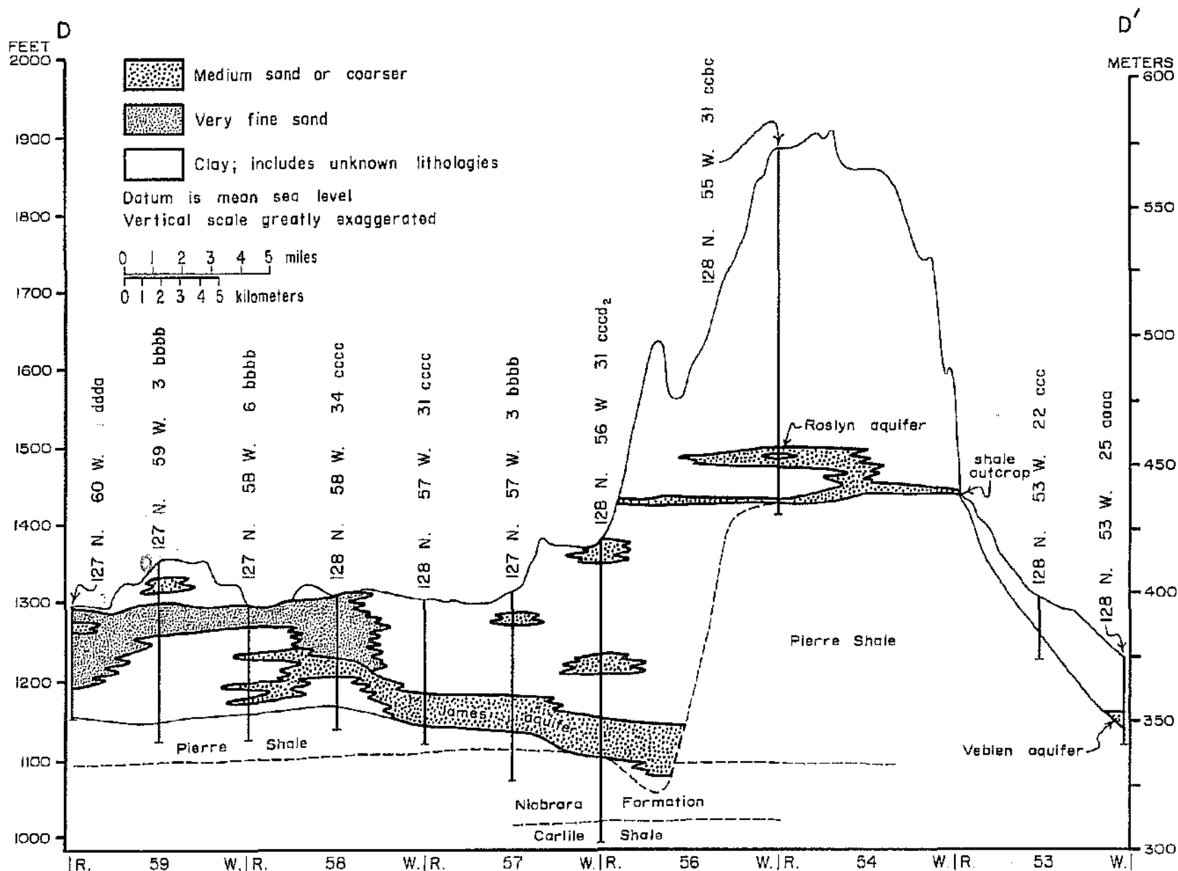
Figure 19 - (D-D'). Lithologic sections B-B' to F-F' showing where major aquifers occur.
