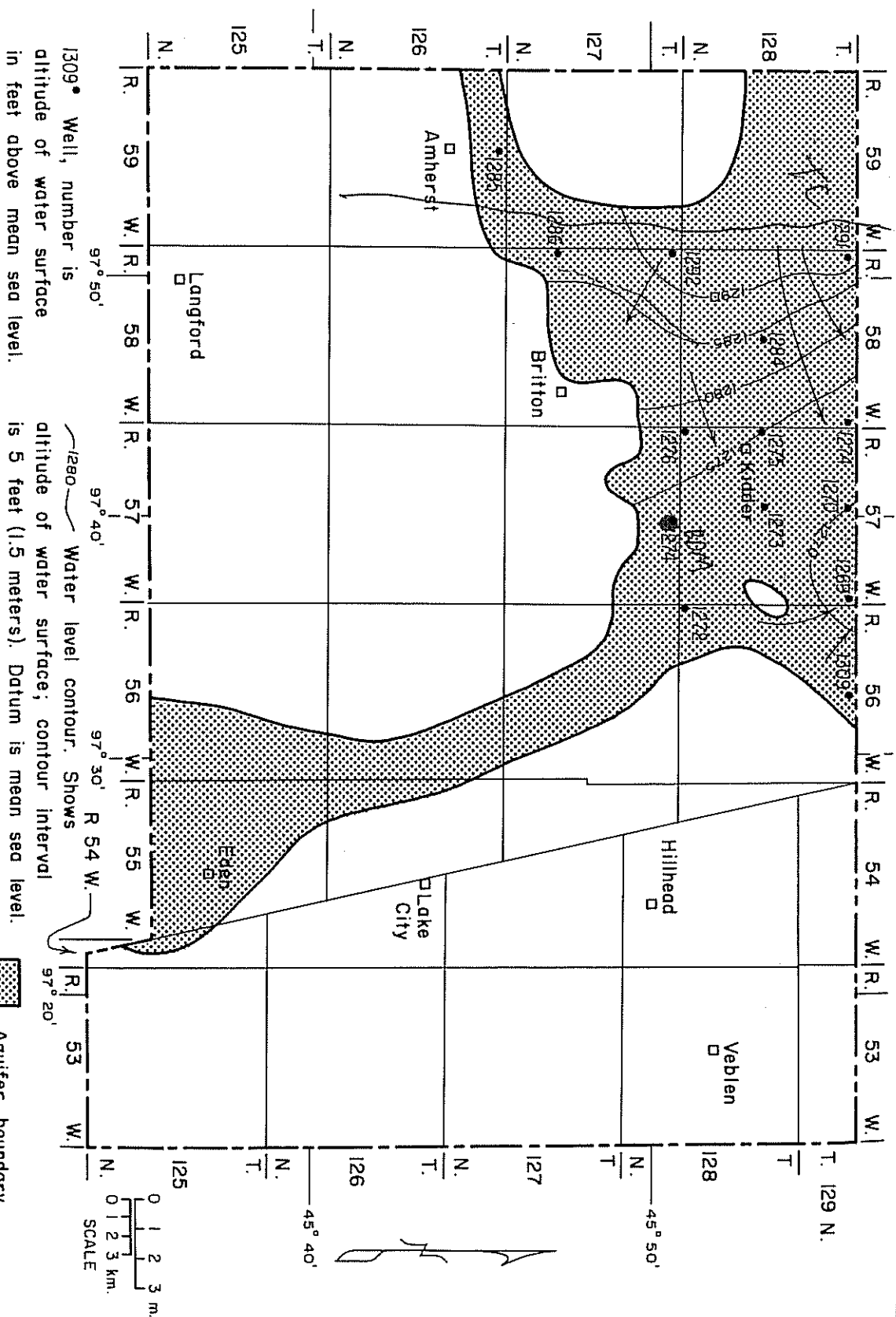
Figure 21. Map showing altitude of the water surface and direction of ground-water movement in the James aquifer, November 1971.
