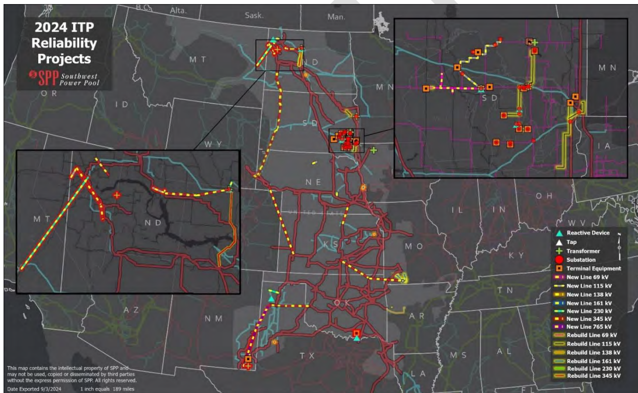
Figure 1.1: 2024 ITP Thermal &amp; Voltage Reliability Projects
