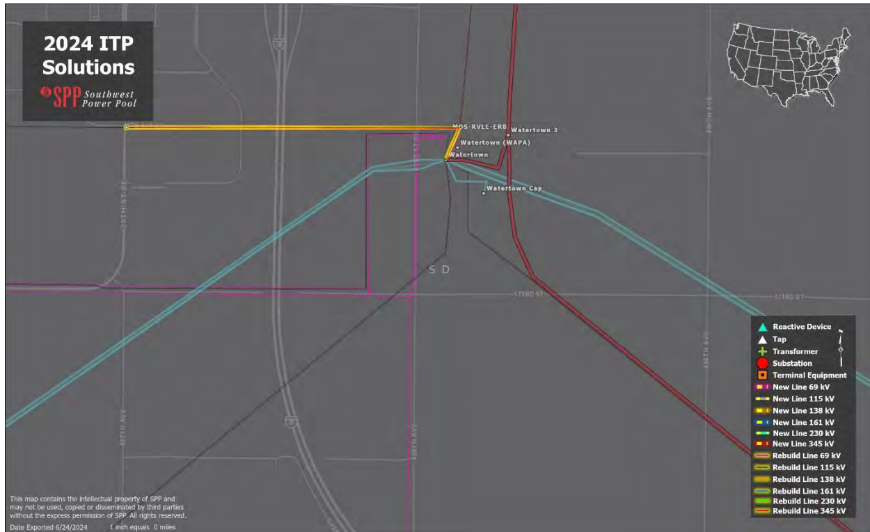
Figure 6.41: UMZ: 15th Ave – Watertown 115 kV Rebuild
