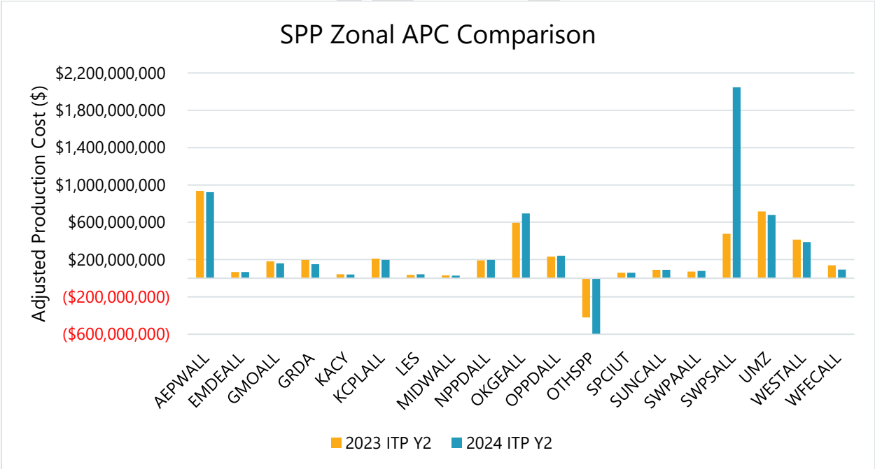
Figure 3.38: SPP Zonal APC Comparison
