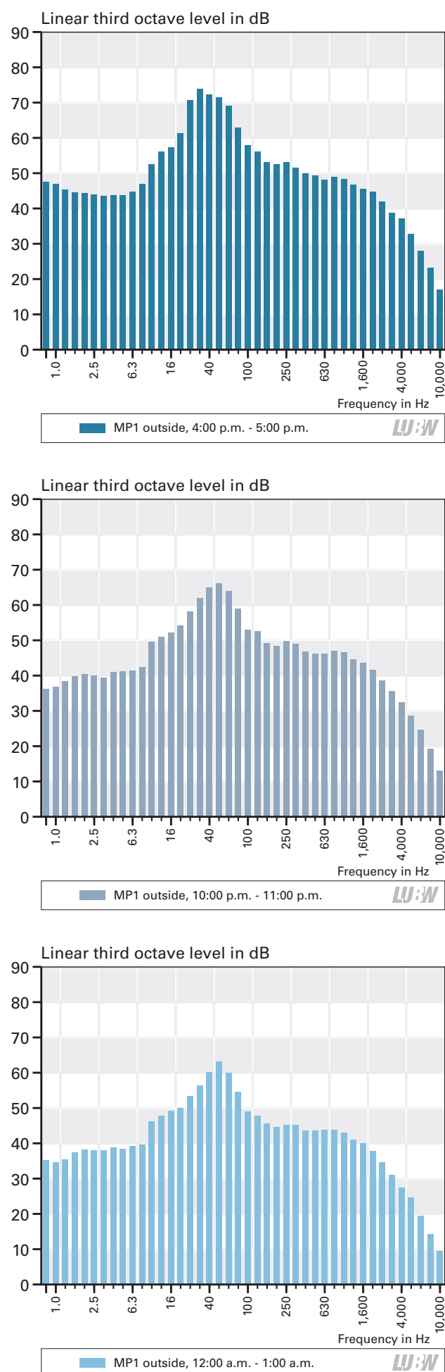
Figure 5.1-3: Linear third octave spectra for the periods 4:00 p.m. - 5:00 p.m. (top), 10:00 p.m. - 11:00 p.m. (centre) and 12:00 a.m. - 1:00 a.m. (below) at the outside measurement point MP1. A significant peak in the frequency range 25 Hz to 80 Hz can be seen for the spectra, which is due to vehicle traffic.
