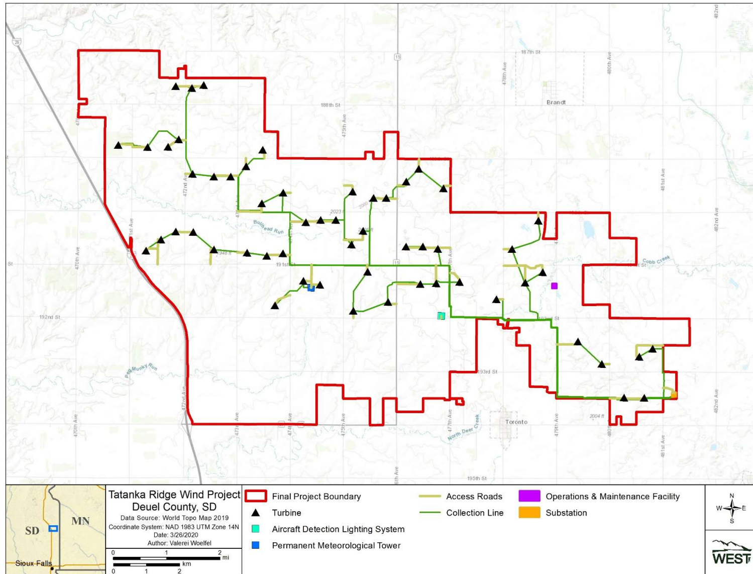
Figure 2. Layout of the Tatanka Ridge Wind Project.
