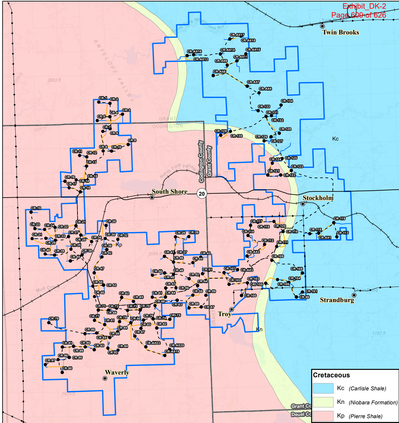
Figure 10. Bedrock Geology
