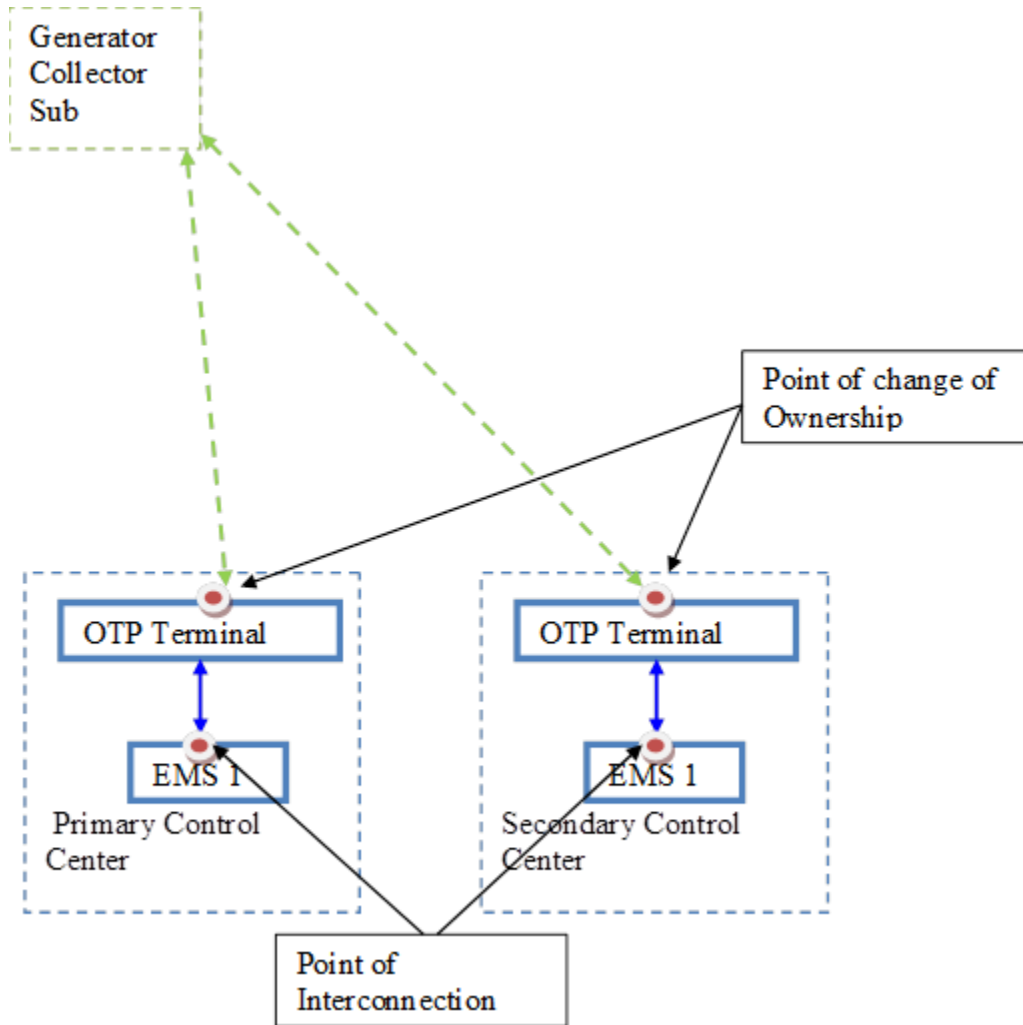
Exhibit A2-2 Communications Block Diagram – circuits to primary and backup Control Center are required
