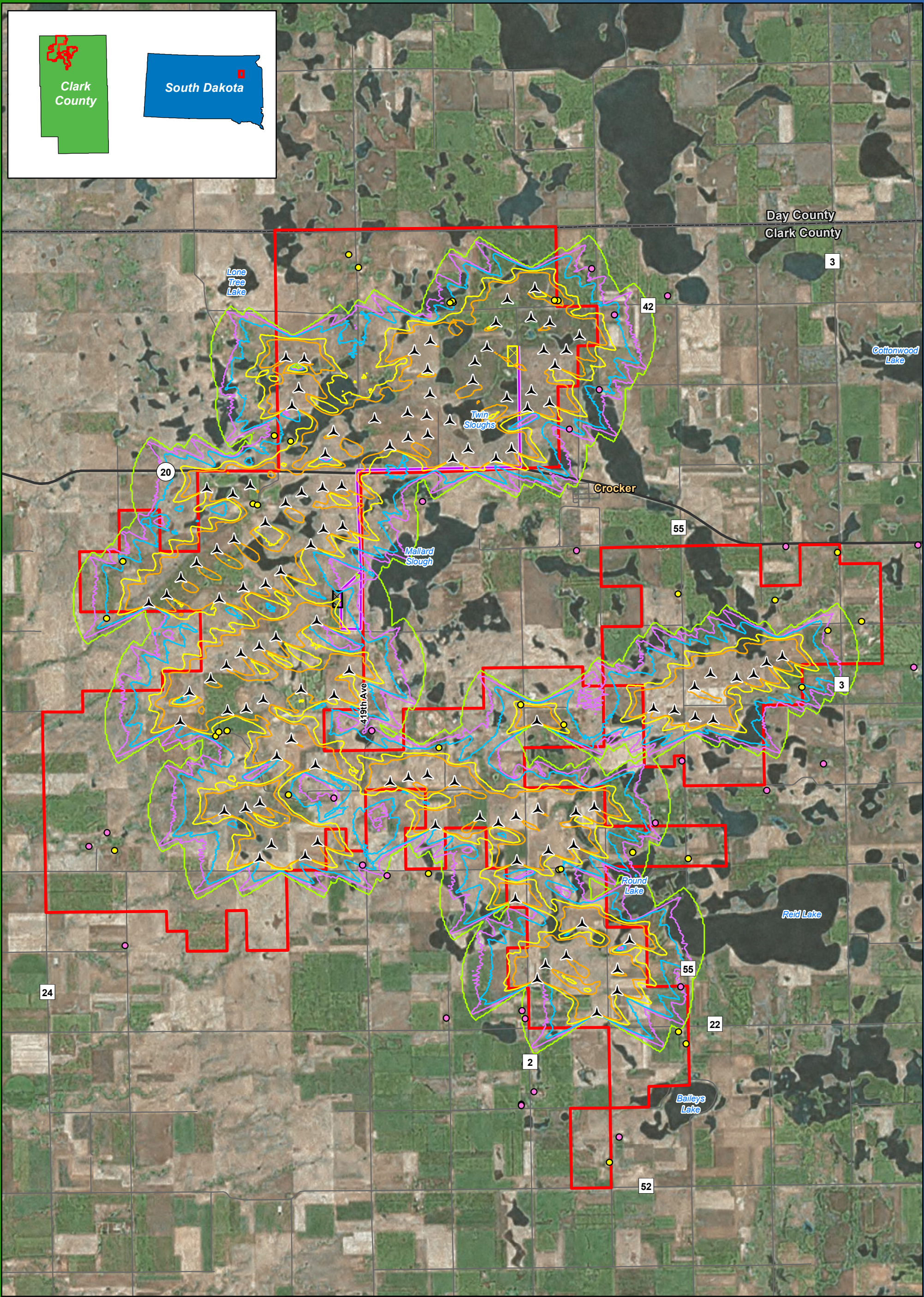
Figure 9b Shadow Flicker Vestas V136 Crocker Wind Farm Clark County, SD 45.079602, -97.845696
