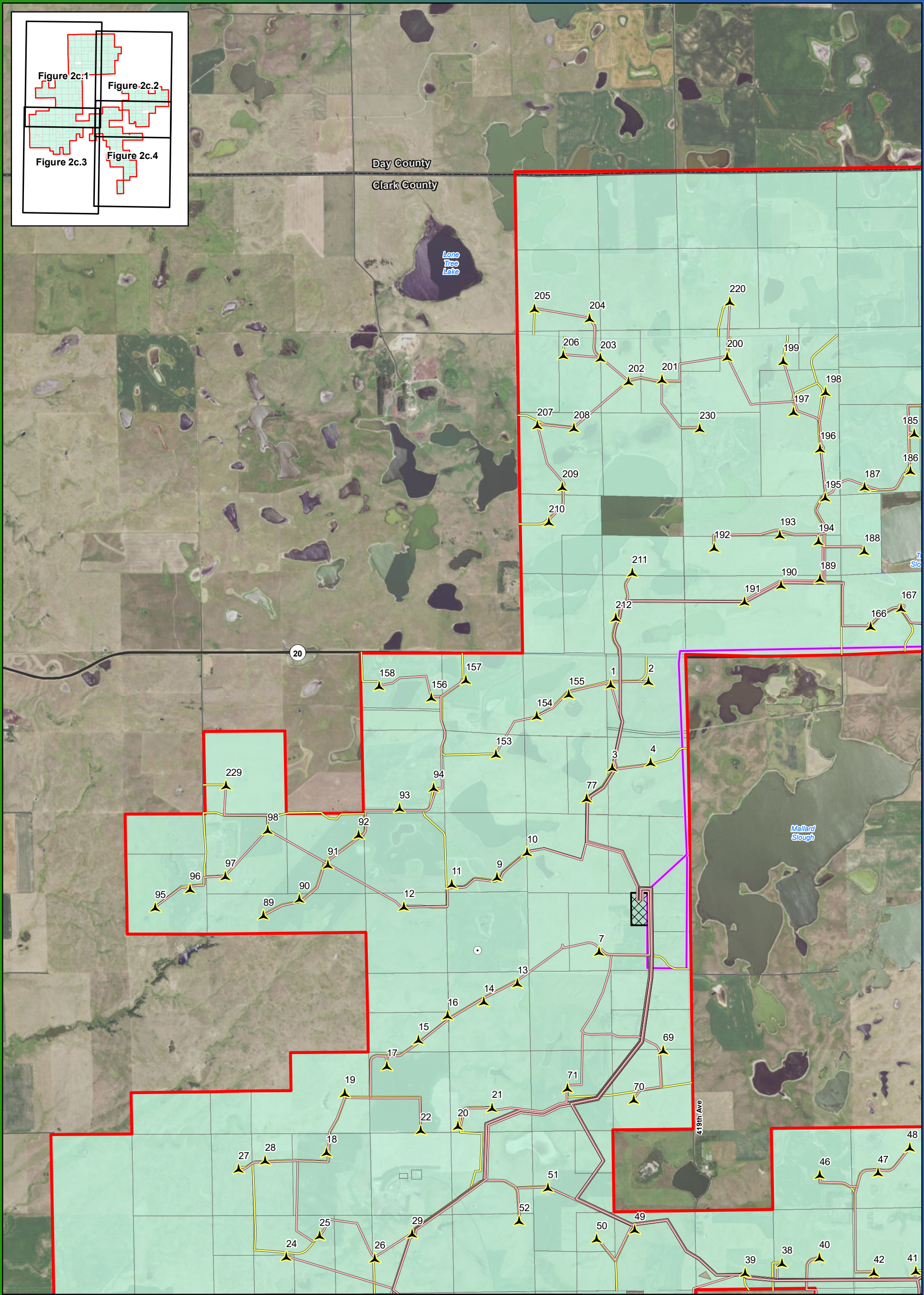
Figure 2c.1 Preliminary Project Layout Map Series GE 2.5-116
