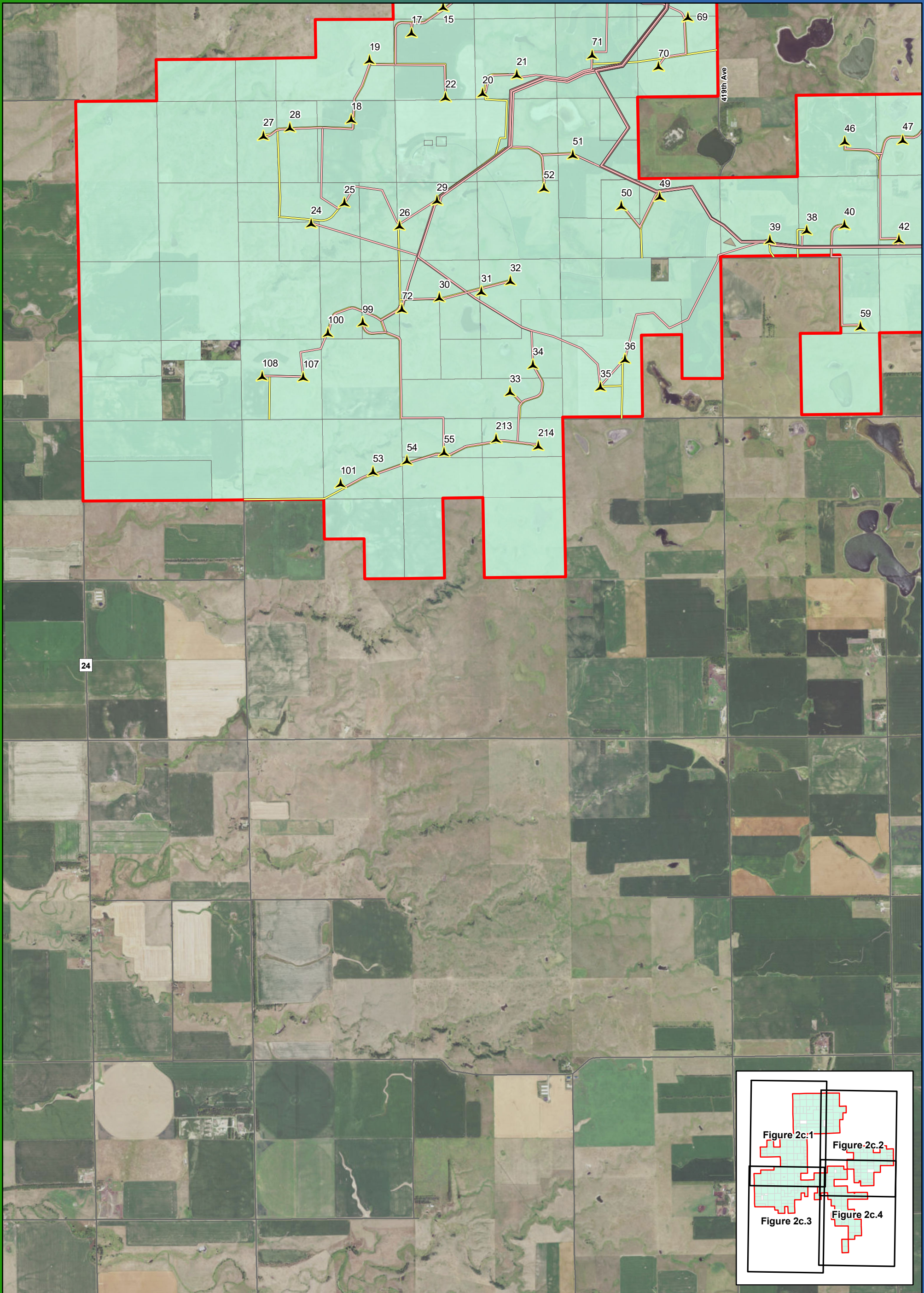
Figure 2c.3 Preliminary Project Layout Map Series GE 2.5-116
