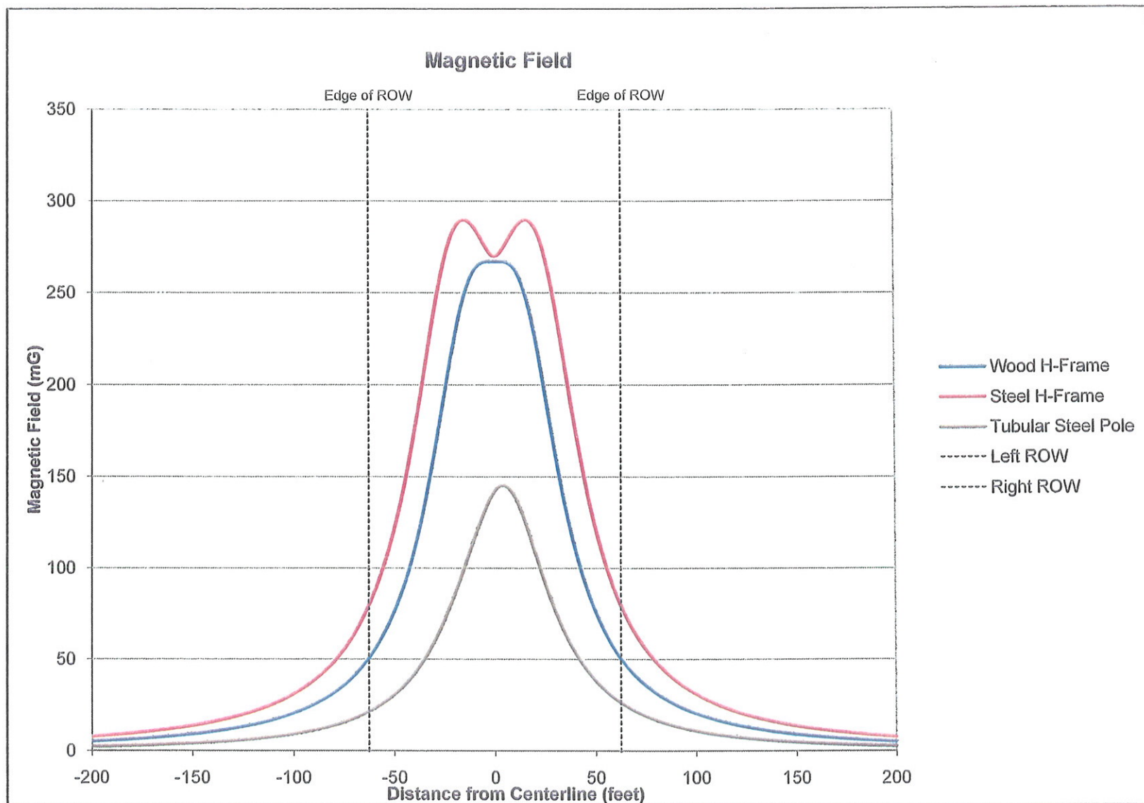
Figure 4: Magnetic Field Plot
