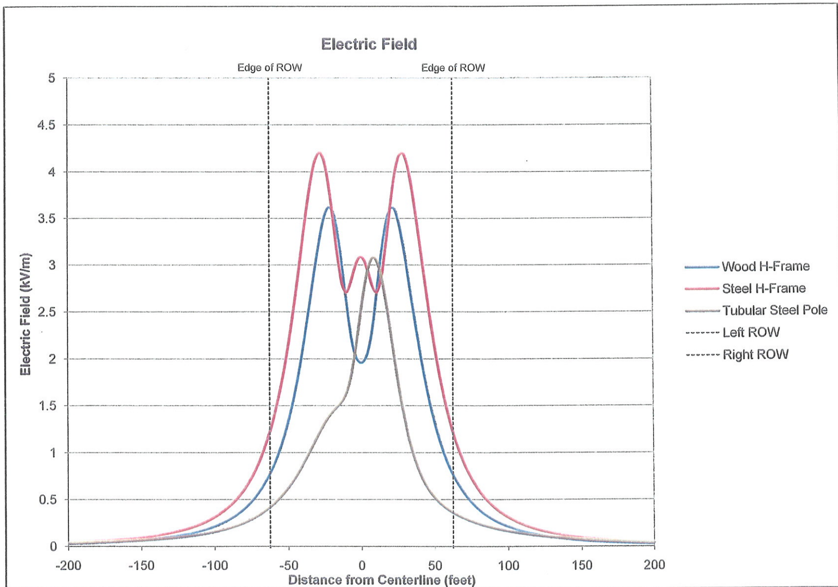
Figure 3: Electric Field Plot
