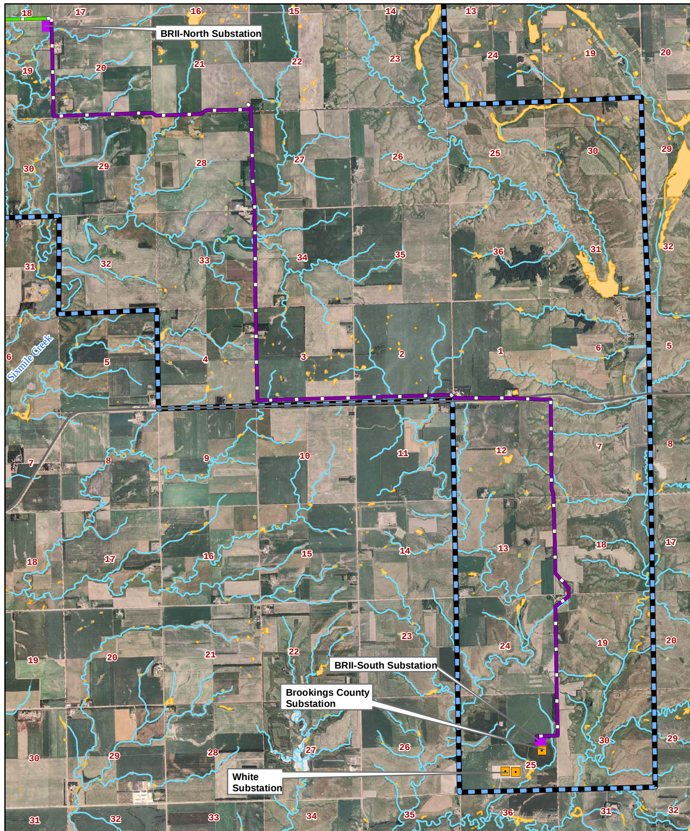
Figure 11b - NWI Wetlands & Streams, 115 kV Transmission Line Buffalo Ridge II Wind Farm Iberdrola Renewables Brookings and Deuel Counties, SD
