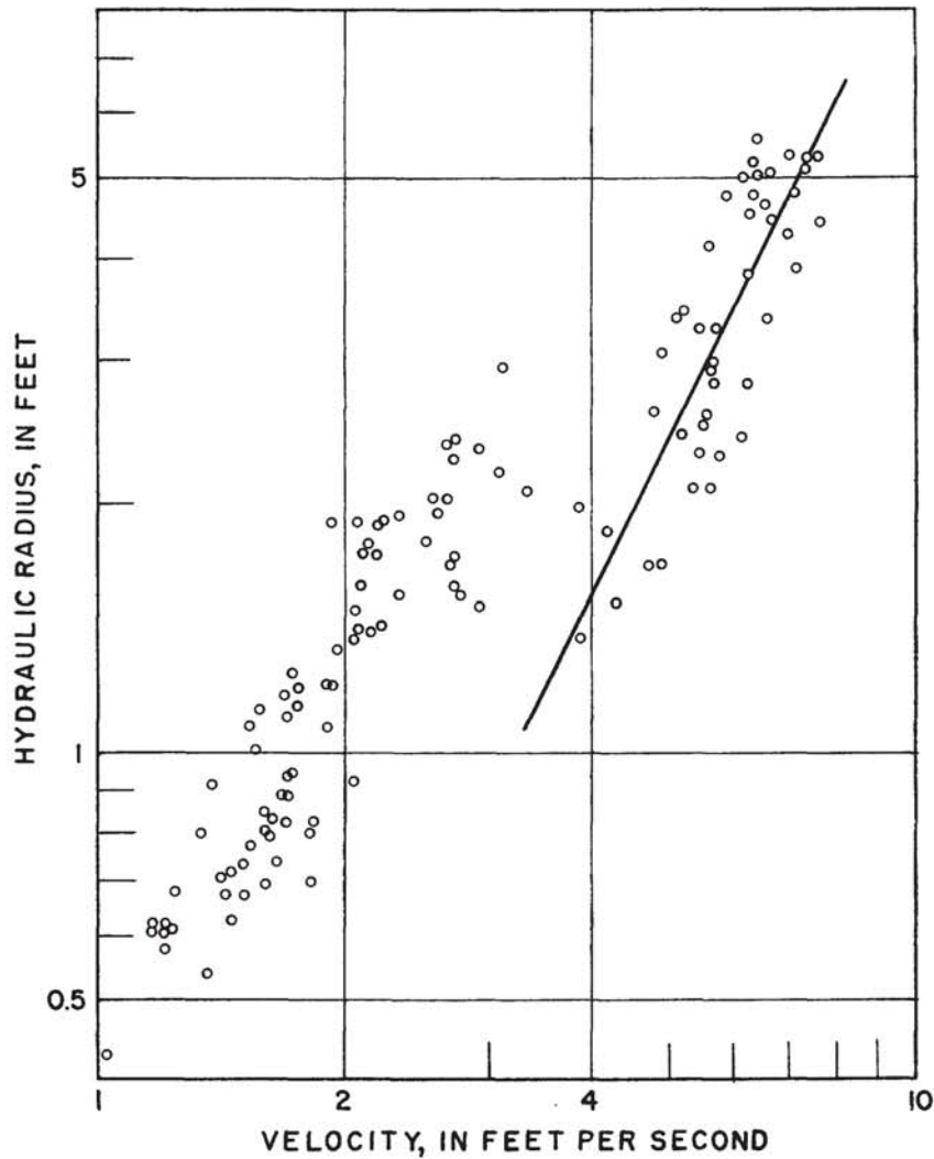
FIGURE 5.—Relation of velocity to hydraulic radius for Pigeon Roost Creek near Byhalla, Miss.
