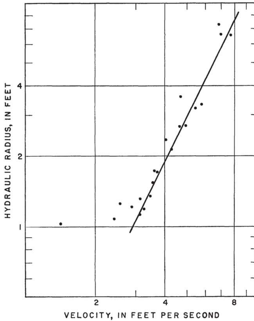
FIGURE 7.—Relation of velocity to hydraulic radius for Cheyenne River near Spencer, Wyo.
