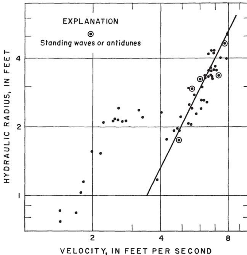
FIGURE 9.—Relation of velocity to hydraulic radius for Rio Grande near Bernalillo, N. Mex.
