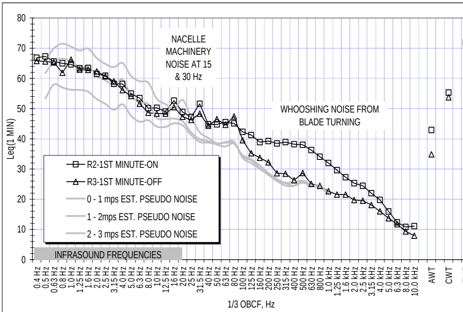
Figure 5.1 On/Off Sound Levels Outdoors during Project Operation
